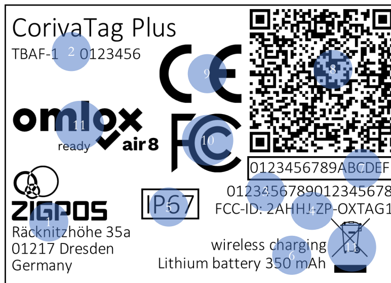
Figure 4 - Example of the CorivaTag Plus nameplate
